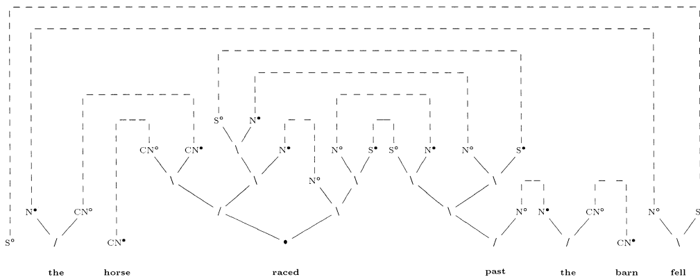
Figure 2 Proof net analysis of (1b) the horse raced past the barn fell .
