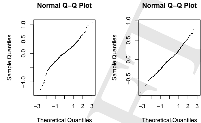
Figure A.17: Quantile-quantile plots for linear mixed-effects models fit to the country data, with \log(\text{Count}) as dependent variable. Left: untrimmed model, right: trimmed model.
