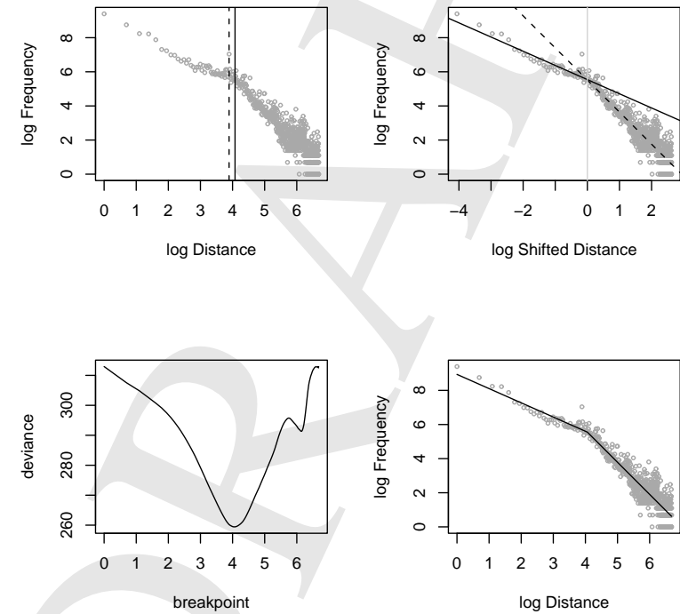
Figure 6.14: Breakpoint analysis of the frequency of use of references to years in the Frankfurter Allgemeine Zeitung in 1994 as a function of the distance of the year name from 1994.
