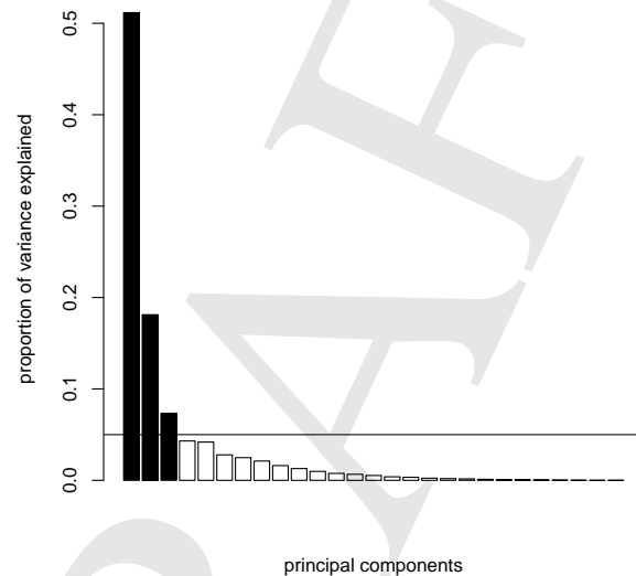
Figure 5.2: Screeplot for the principal components analysis of texts in affix productivity space.
