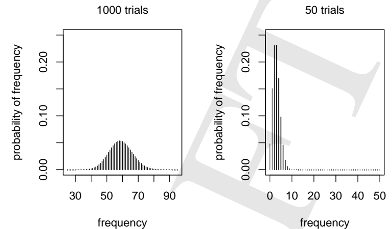
Figure 3.2: The frequencies (horizontal axis) and the probabilities of these frequencies (vertical axis) for the assuming that its frequency is binomially distributed with p = 0.05885575 and n = 1000 (left panel) or n = 50 (right panel).
