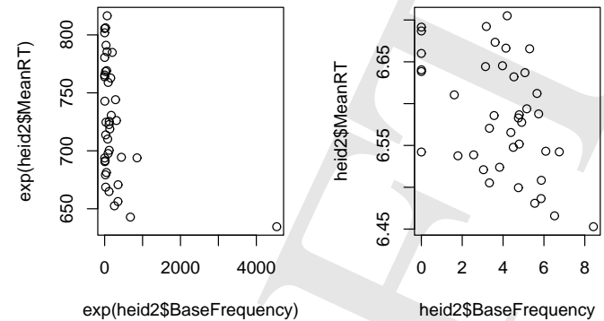
Figure A.2: Scatterplots of reaction time in visual lexical decision by base frequency for neologisms in -heid without (left) and with (right) logarithmically transformed variables. Note that without the log transformation, the pattern in the data is dominated by just one word with a very high base frequency.
