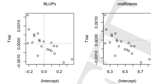
Figure 7.4: Best linear unbiased predictors (BLUPs) for the by-subject random effects for model lexdec3.lmerD (left panel), and the corresponding by-subject coefficients (right panel).
