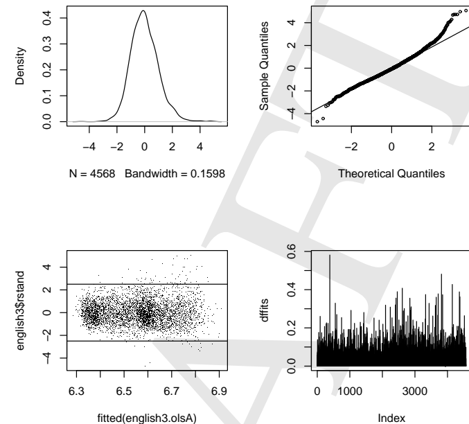
Figure 6.9: Model criticism for english3.olsA : a density plot of the standardized residuals (upper left), the corresponding quantile-quantile plot (upper right), standardized residuals by predicted reaction time (lower left), and dffits (lower right).
