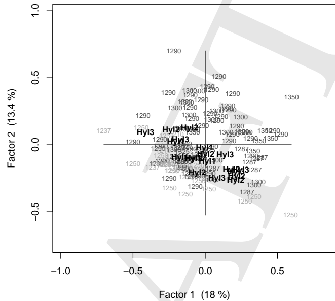
Figure 5.7: Correspondence analysis of the frequencies of 35 tag trigrams in 125 Old French prose fragments. Text fragments are labeled by approximate date of origin, texts dating from 1250 or earlier are shown in light grey, texts located later in time are shown in dark grey. The texts in black represent supplementary rows representing texts of unknown date.
