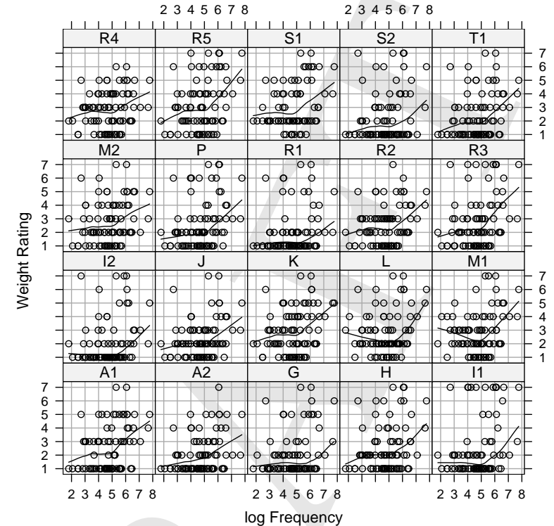
Figure 2.10: Weight rating as a function of log word frequency grouped by subject.
