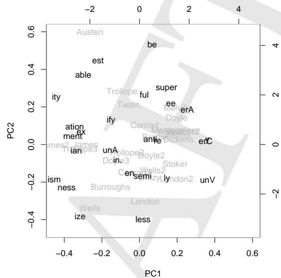
Figure A.9: Biplot for texts and affixes, the second principal component captures year of birth.
