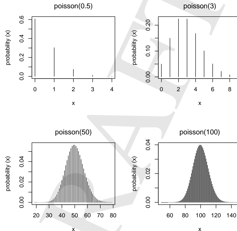
Figure 3.4: Poisson frequency functions for \lambda = 0.5, 3, 50, 100 .
