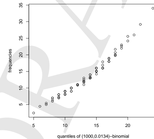
Figure 3.3: Quantile-quantile plot for inspecting whether the frequency of the definite article the in the Dutch novel Max Havelaar is binomially distributed.
