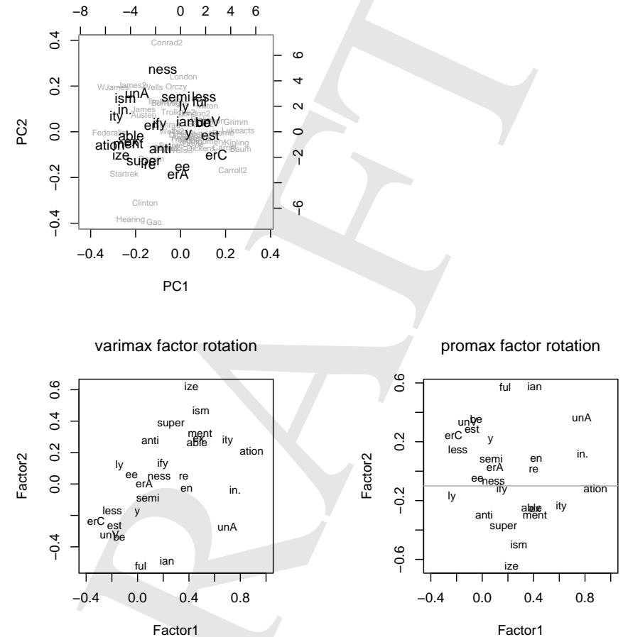
Figure 5.5: Upper panel: Biplot for the principal components analysis of texts and affixes based on productivity scores, now using the correlation matrix instead of the covariance matrix. Lower panel: The loadings of the affixes on the first two factors in a factor analysis using varimax (left) and promax factor rotation.
