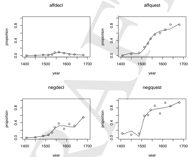
Figure 6.15: The relative frequency of periphrastic do in four sentence types across three ages. Circles represent observed relative frequencies, dashed and solid lines a regression model without and with an indicator variable adjusting for the fifteenth century.
