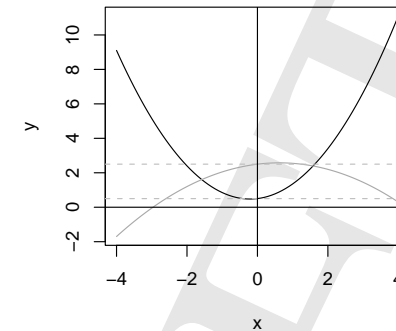
Figure 4.13: Two parabola.
