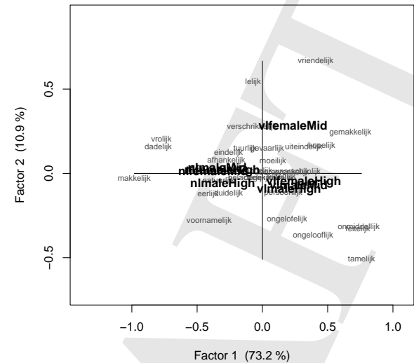
Figure 5.8: Correspondence analysis of the frequencies of 32 words ending in the Dutch suffix -lijk in 8 subcorpora of spoken conversational Dutch.
