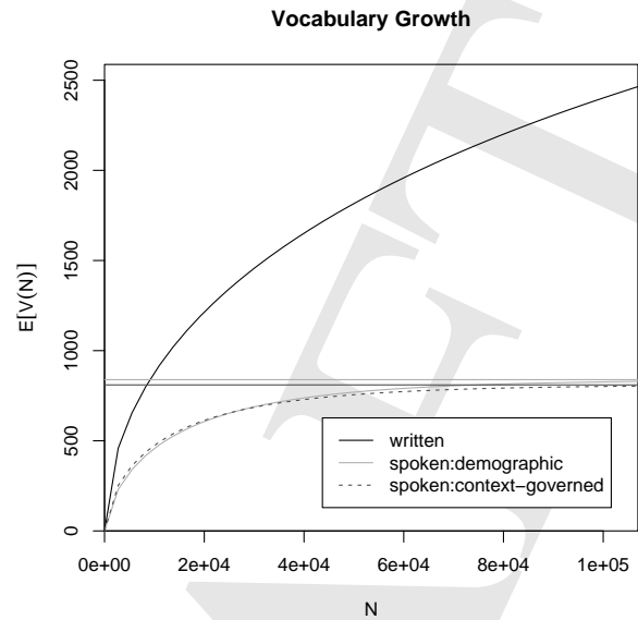
Figure A.15: The growth curve of the vocabulary for the English suffix -ness in the three main subcorpora of the British National Corpus.
