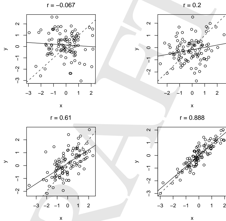
Figure 4.10: Scatterplots for four paired standard normal random variables with different population correlations ( \rho = 0.0, 0.2, 0.5, 0.9 ). The correlations shown above each panel are the sample correlations.
