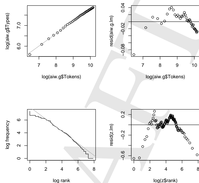
Figure 6.17: Herdan's law (upper left) and Zipf's law (lower left) and the corresponding residuals (right panels) for Alice's Adventures in Wonderland .
