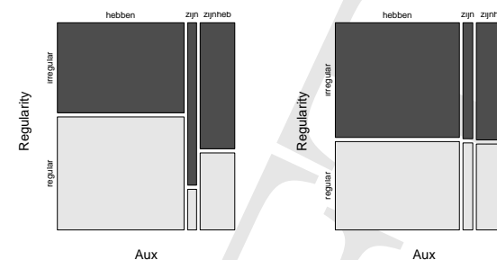
Figure 4.17: Mosaic plots for Dutch verbs cross-classified by regularity and auxiliary (left panel) and a fictitious data set (right panel).
