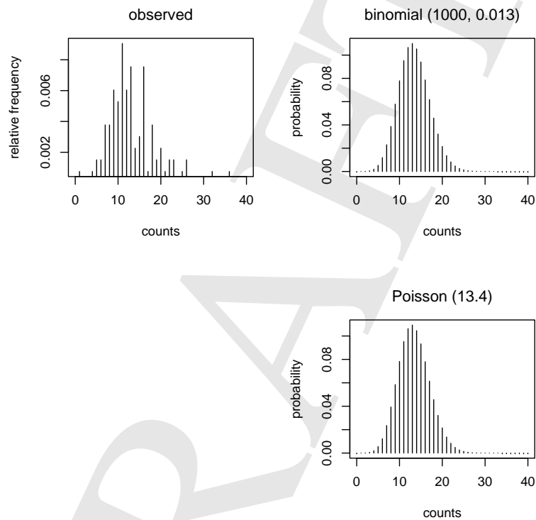
Figure 3.5: Observed relative frequencies of the definite article het ('the') in sequences of 1000 word tokens in the novel Max Havelaar and the corresponding binomial and Poisson distributions.
