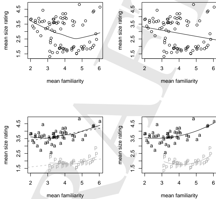
Figure 4.12: Scatterplots for mean rated size as a function of mean familiarity, with scatterplot smoothers (left panels) and linear (upper right, lower left) and quadratic (lower right) fits. The upper panels show fits to all data points, the lower panels show fits to the words for plants (p) and animals (a) separately.
