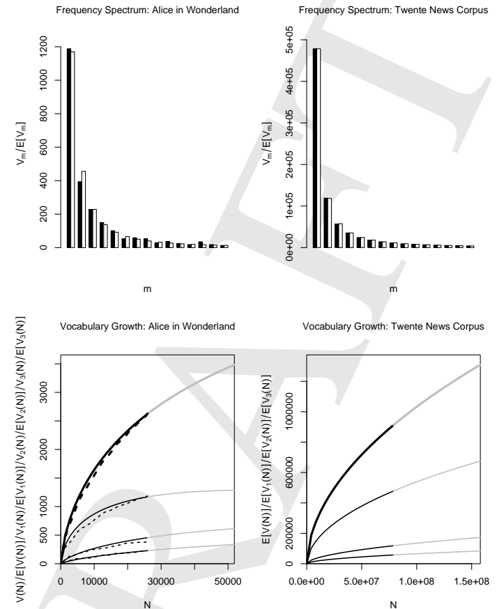
Figure 6.19: Observed (black) and expected (white) frequency spectrum for Alice's Adventures in Wonderland and the Twente News Corpus (upper panels) and the corresponding vocabulary growth curves (lower panels). For the growth curves, black lines represent interpolation, grey lines extrapolation to twice the observed sample size, and dashed lines the observed growth curves (only available for Alice's Adventures in Wonderland ).
