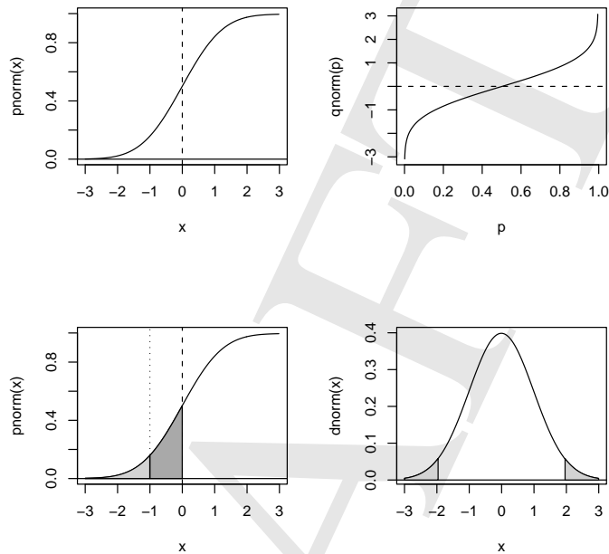
Figure 3.7: Cumulative distribution function (left panels), quantile function (upper right panel), and probability density function (lower right panel) for the standard normal distribution.
