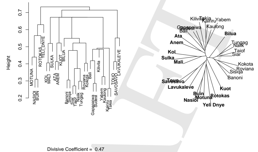
Figure 5.12: Divisive clustering with diana() (in the cluster package) and the corresponding unrooted tree obtained with the neighbor-joining algorithm nj() (in the ape package) of 16 Oceanic and 15 Papuan languages using 125 grammatical traits [Dunn et al., 2005].
