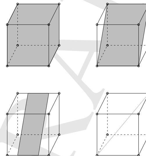
Figure 5.1: Different distributions of points (highlighted in grey) in a cube.
