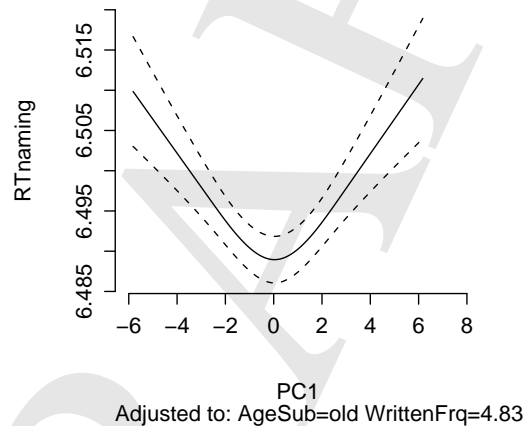
Figure A.12: The partial effect of PC1 on the naming latencies in the english data set.
