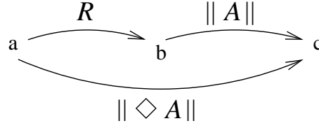
Fig. 2: Horizontal dynamic interpretation of \diamond A
